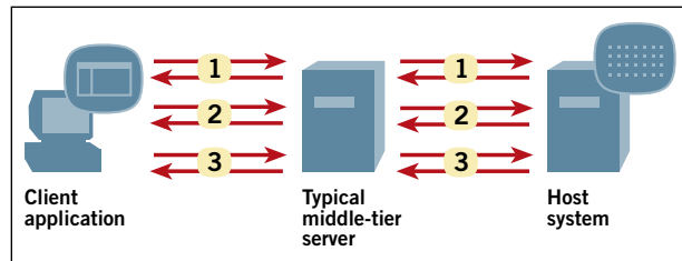
Figure 6: Network Traffic Generated by Low-Level APIs
